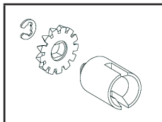
No. 505071 Kegelzahnrad B Differential Differential bevel gear set
